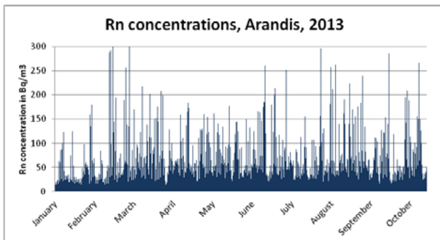
Figure 33: Radon concentrations at the Arandis radon monitoring station, for the year 2013.
