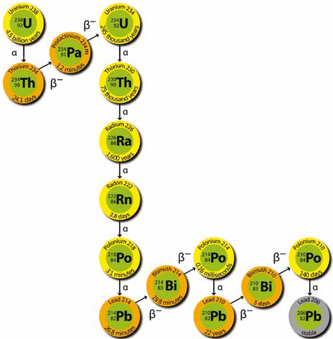
Figure 48: U-238 principal decay modes, with permission from VO Consulting, www.voconsulting.net
