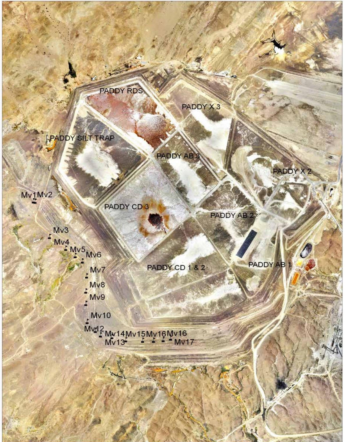
Figure 37: Location of multi-vertical samplers on TSF.
